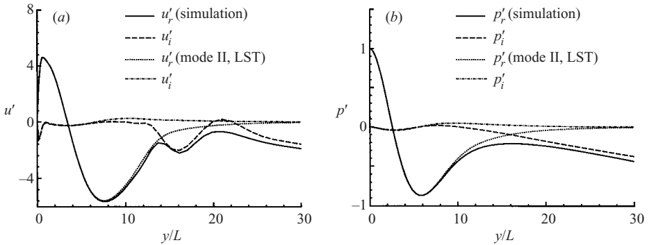
FIGURE 8. Comparison of the wave structures of disturbances induced by free-stream fast acoustic waves and those of mode II obtained by the linear stability theory at R = 1614.43 ( F = 2.2 \times 10^{-4} and \theta_\infty = 0^\circ ).
