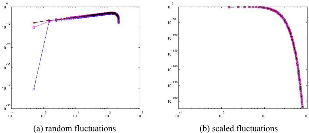
Figure 3: Spectra of fluctuations of flow variables.
