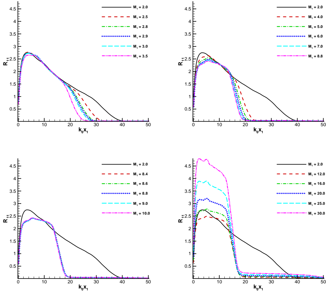
Figure 8: Evolutions in streamwise-streamwise Reynolds stresses for inflow conditions of case I.
