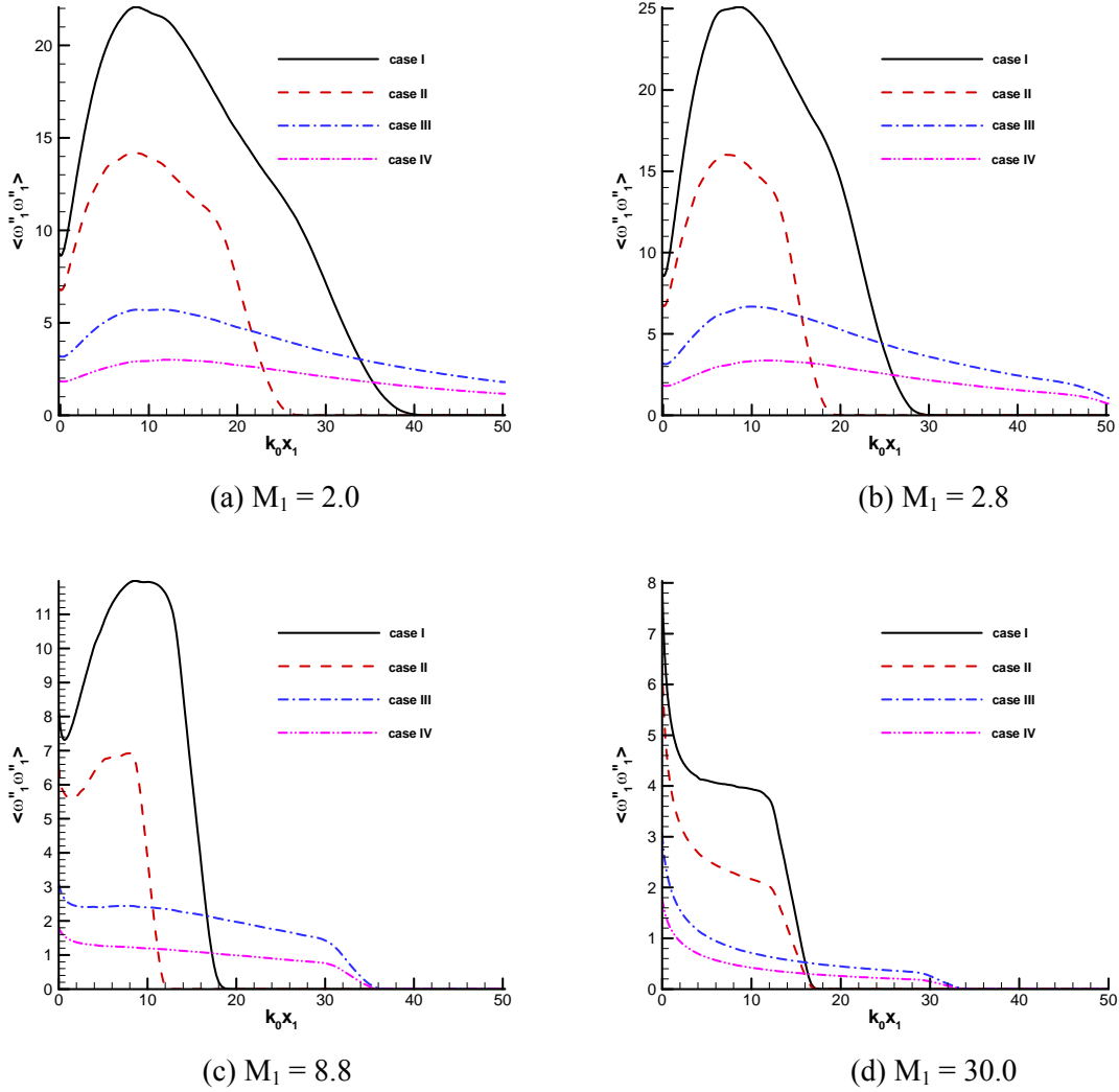
Figure 7: Variance of streamwise vorticity fluctuations at a given shock Mach number.
