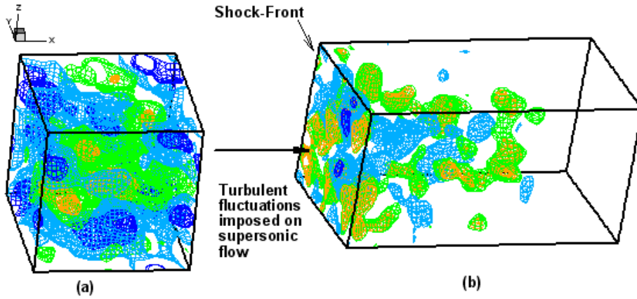
Figure 2: Schematic showing typical density contours and computational domains for simulation of shock-turbulence interaction using shock-fitting algorithm [1].
