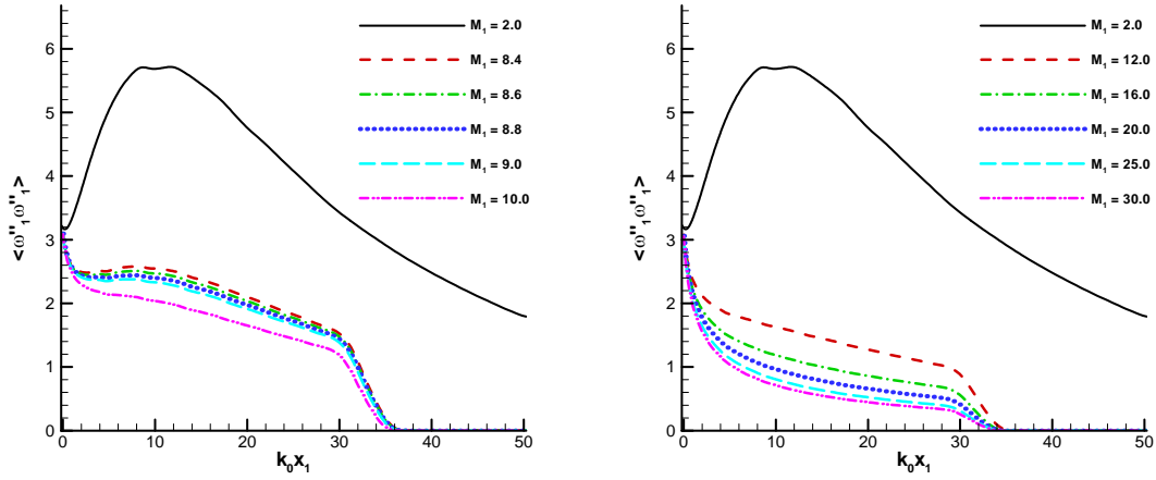
Figure 6: Effect of increasing mean Mach number on the variance of streamwise vorticity for inflow conditions of case III.
