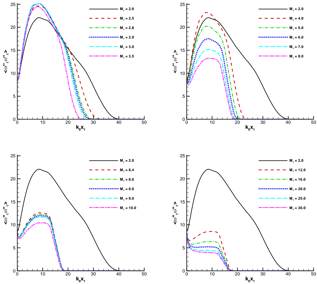
Figure 5: Effect of increasing mean Mach number on the variance of streamwise vorticity for inflow conditions of case I.
