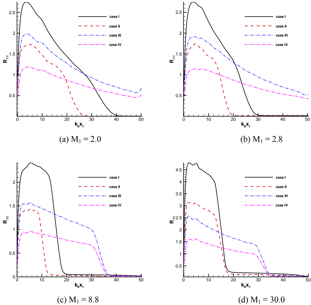
Figure 10: Evolutions in streamwise-streamwise Reynolds stresses at a given shock Mach number.
