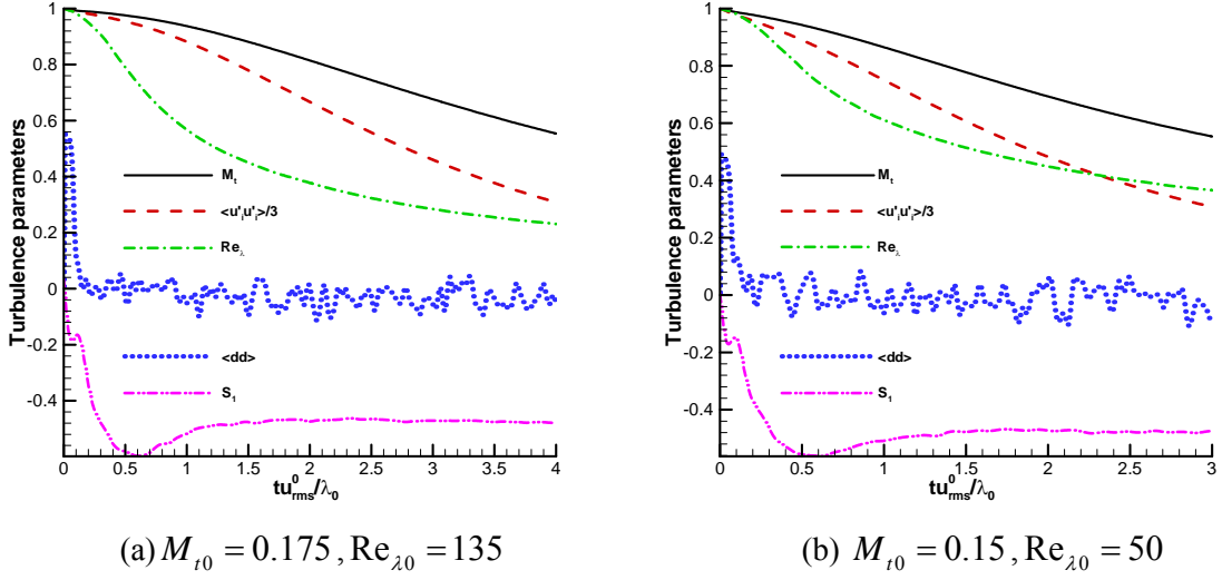
Figure 4: Variation of various turbulence statistics in simulation of decaying isotropic turbulence.
