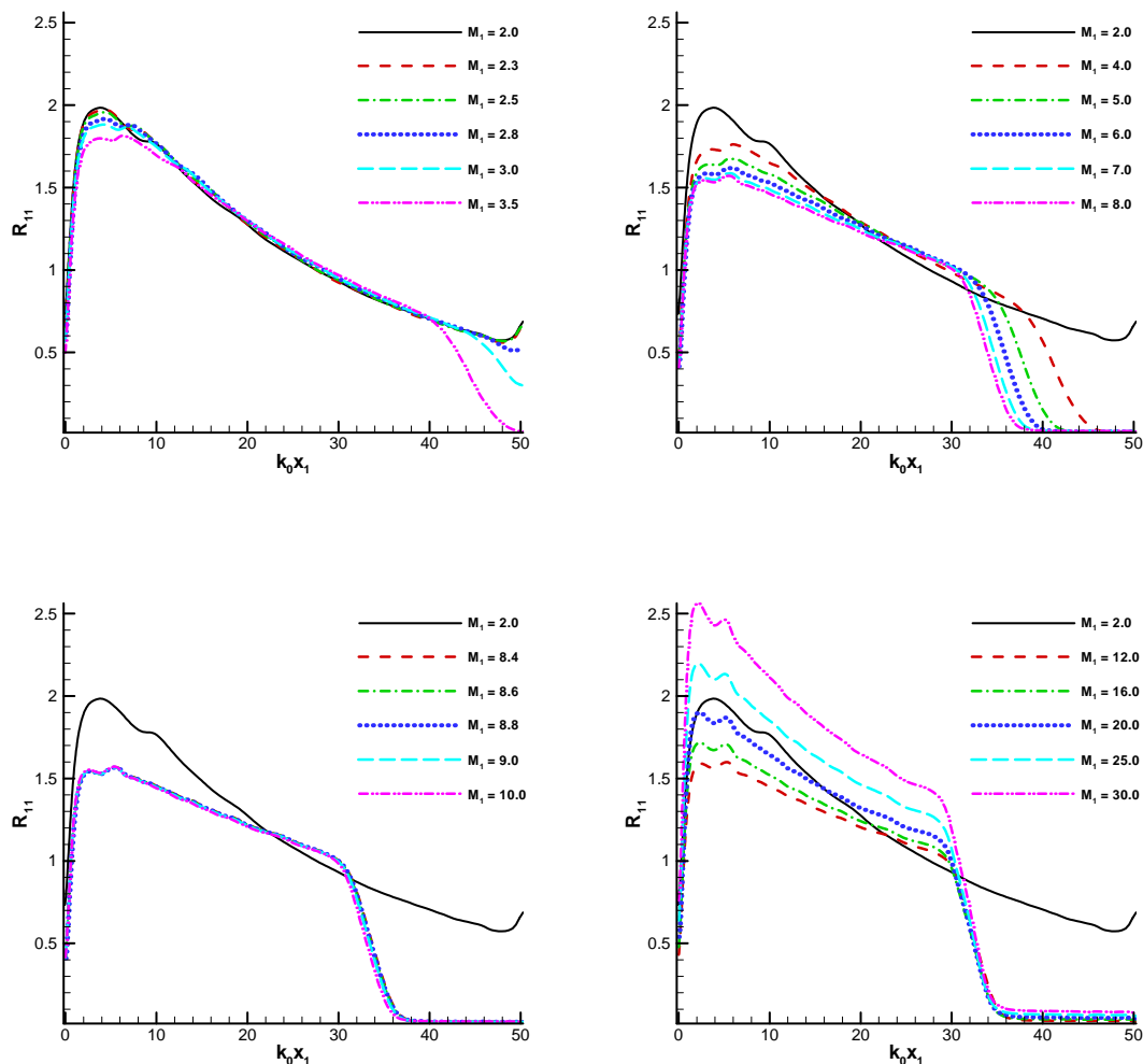
Figure 9: Evolutions in streamwise-streamwise Reynolds stresses for inflow conditions of case III.
