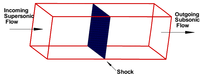
Figure 1: A schematic of canonical strong shock and turbulence interaction problem [1].
